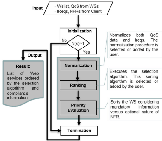
Figure 1. Flow diagram for the web services selection process
