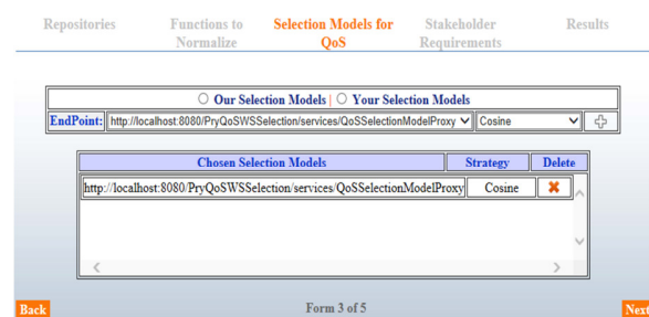
Figure 7. Ranking algorithms interface
