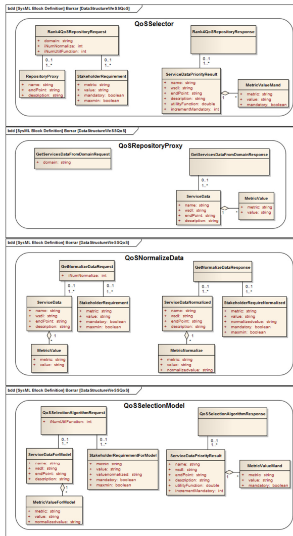
Figure 4. Class diagram of the services supporting the internal architecture of WeSSQoS
