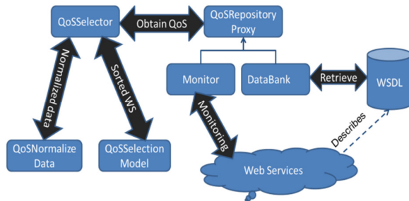
Figure 2. WeSSoS general architecture
