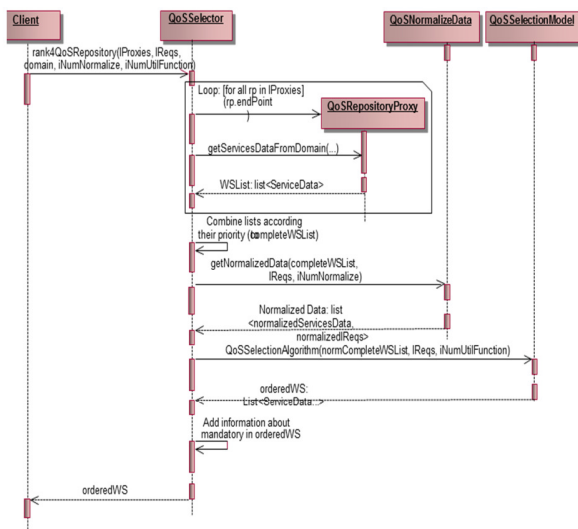
Figure 3. Sequence diagram of the basic use case of the framework
